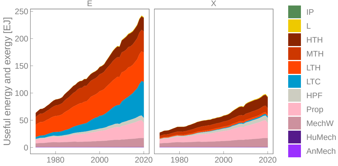
Figure 1: Remake of Figure 7 of the database paper using pre-aggregated (i.e., Grouped) data.
