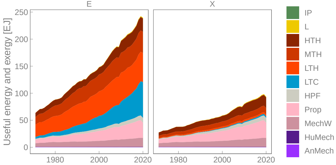
Figure 2: Remake of Figure 7 from the database paper starting from Specified data.
