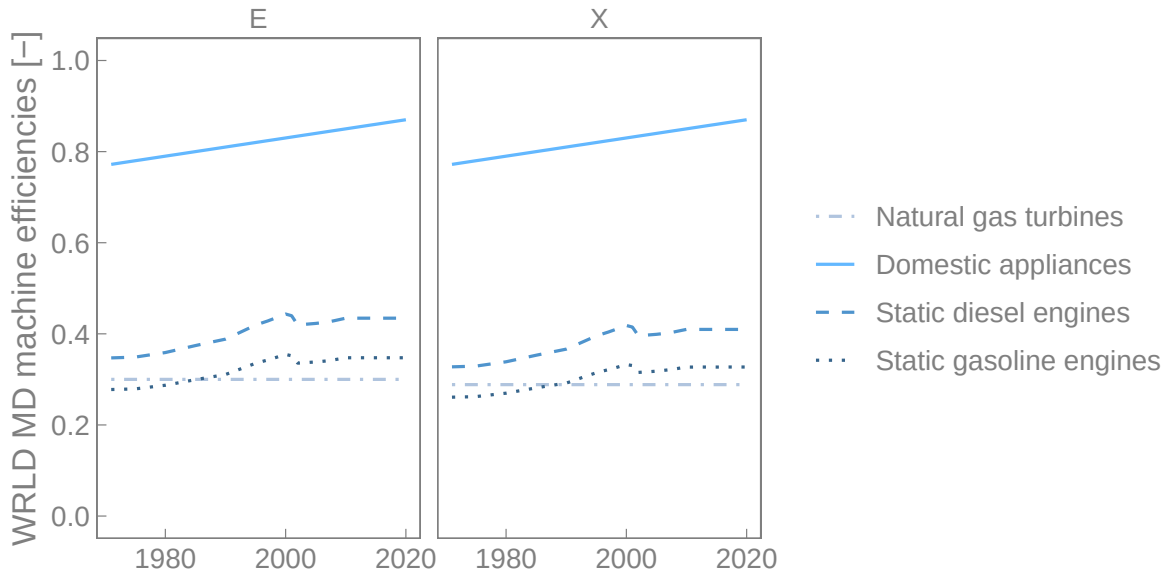
Figure 8: World-level efficiencies of machines that produce MD.
