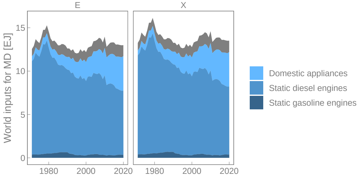
Figure 7: World inputs for mechanical drive (MD) by machine.
